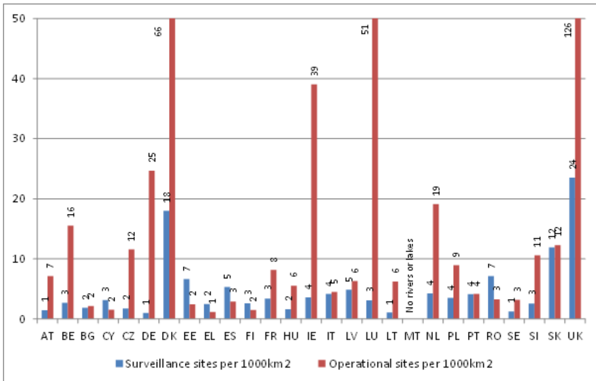
Figure 8.3.3: Number of surveillance and operational monitoring sites for rivers and lakes per 1000 km 2 area (some sites may be for both surveillance and operational monitoring)
