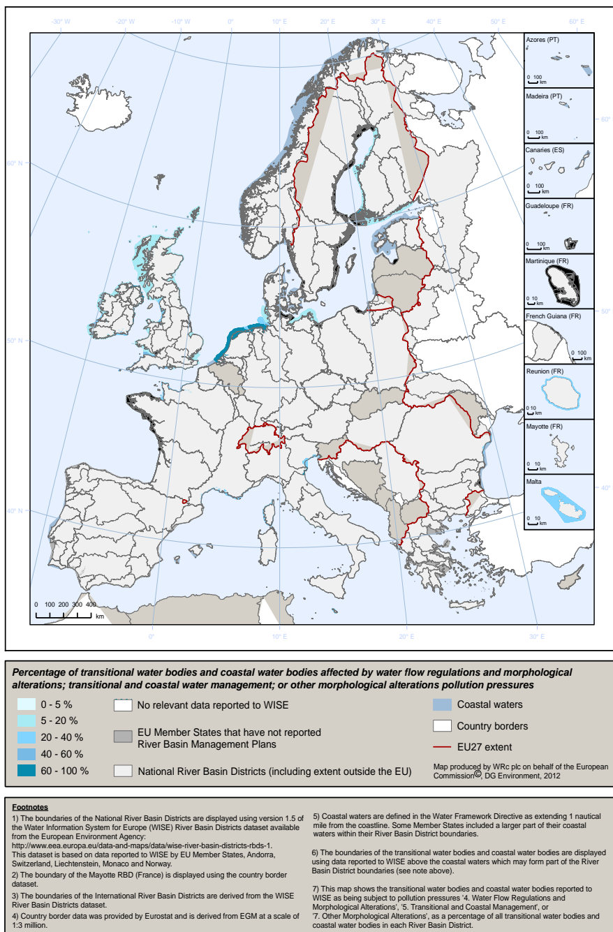
Figure 8.2.9: Proportion of classified water bodies in different River Basin Districts affected by hydromorphological pressures for coastal and transitional waters
